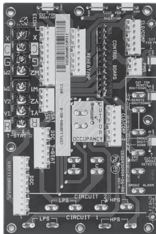
Fig. 31 — Central Terminal Board (CTB)
