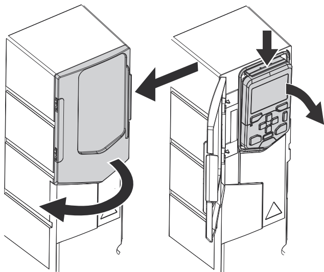
Fig. 45 — Open Keypad Cover and Remove Keypad
