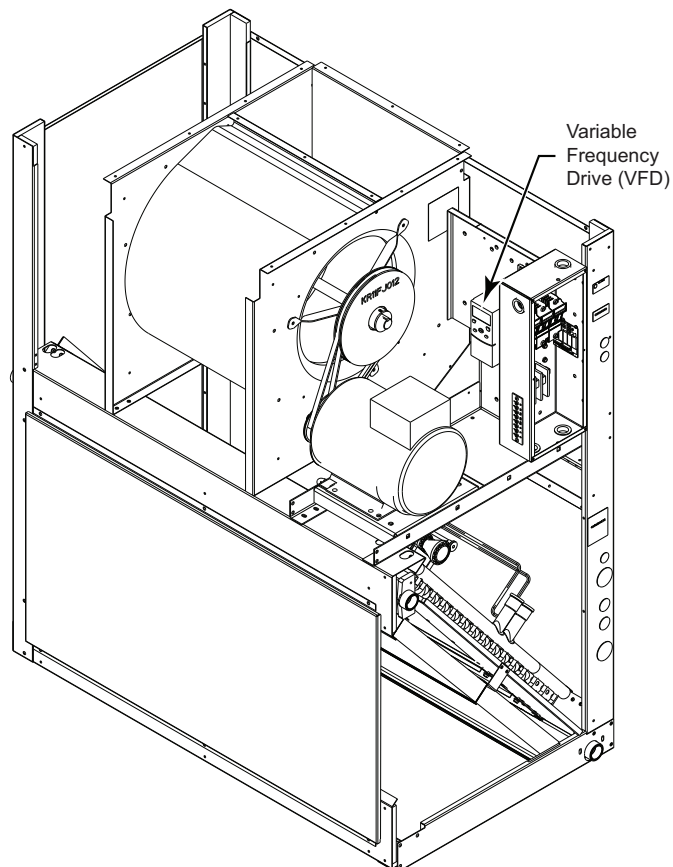
Fig. 18 — ACS320 VFD Location for the following units: 40RUA/RUQ 07-12, 40RUS 08-12 (208/230V and 460V only)
