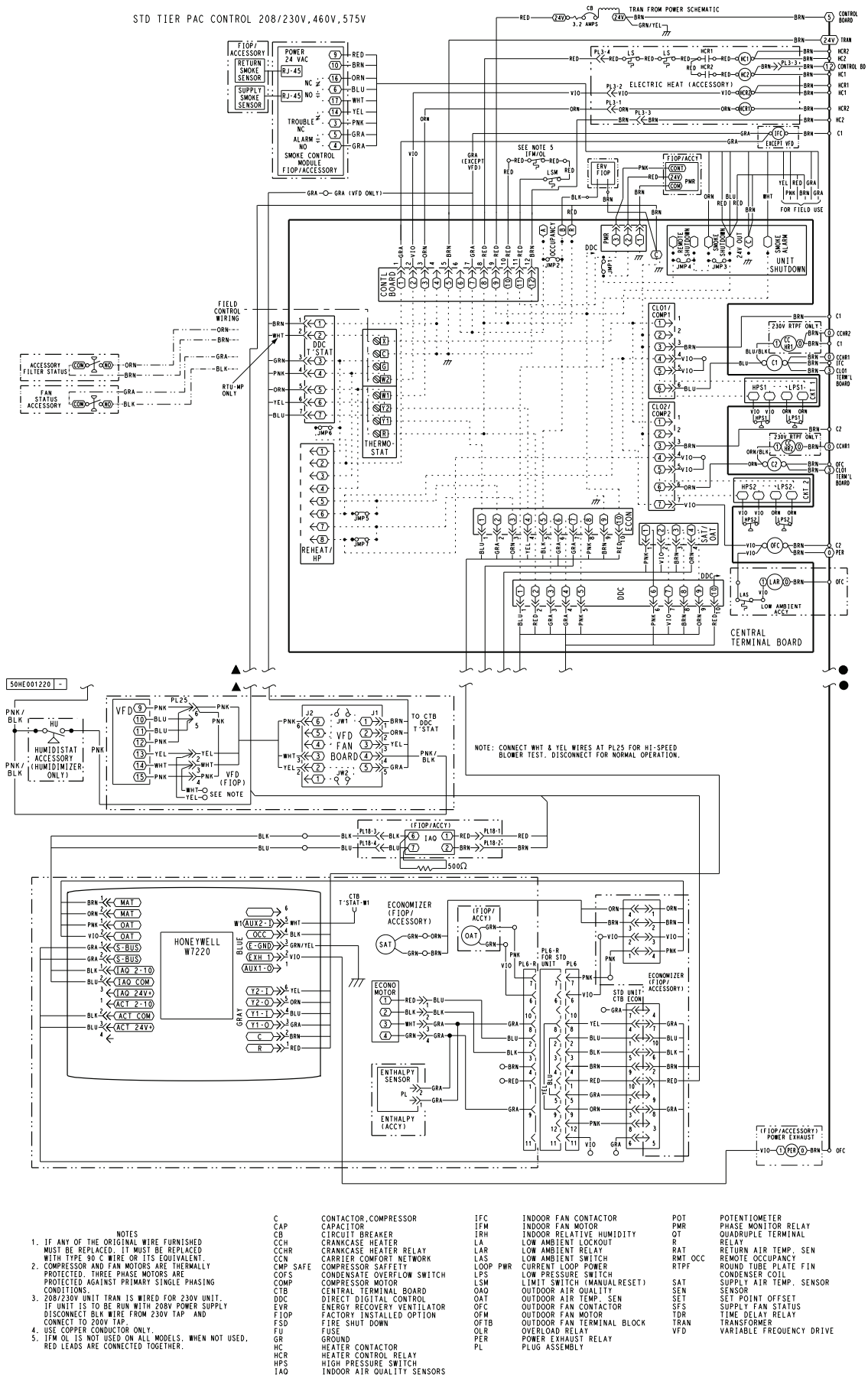
Fig. 37 — Typical Wiring Diagram - Single Package Rooftop Unit (50TC*17-30 and 50HC*17-28 no Comfort Link with ACS320 VFD shown)
