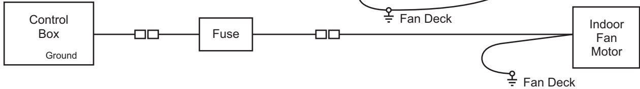
Fig. 51 — To Bypass ACS320 VFD on Fused Units — 48/50TC 07-14, 50TCQ 07-12, 48/50HC 07-12, 50HCQ 08-09 and 40RU Units
