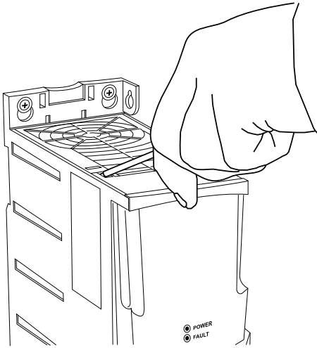
Fig. 42 — Remove Top Cover on ACS320 VFD
