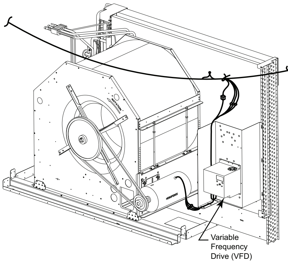
Fig. 14 — ACS320 VFD Location for the following units: 48/50TC 16 and 50TCQ 14 (208/230V and 460V units only)
