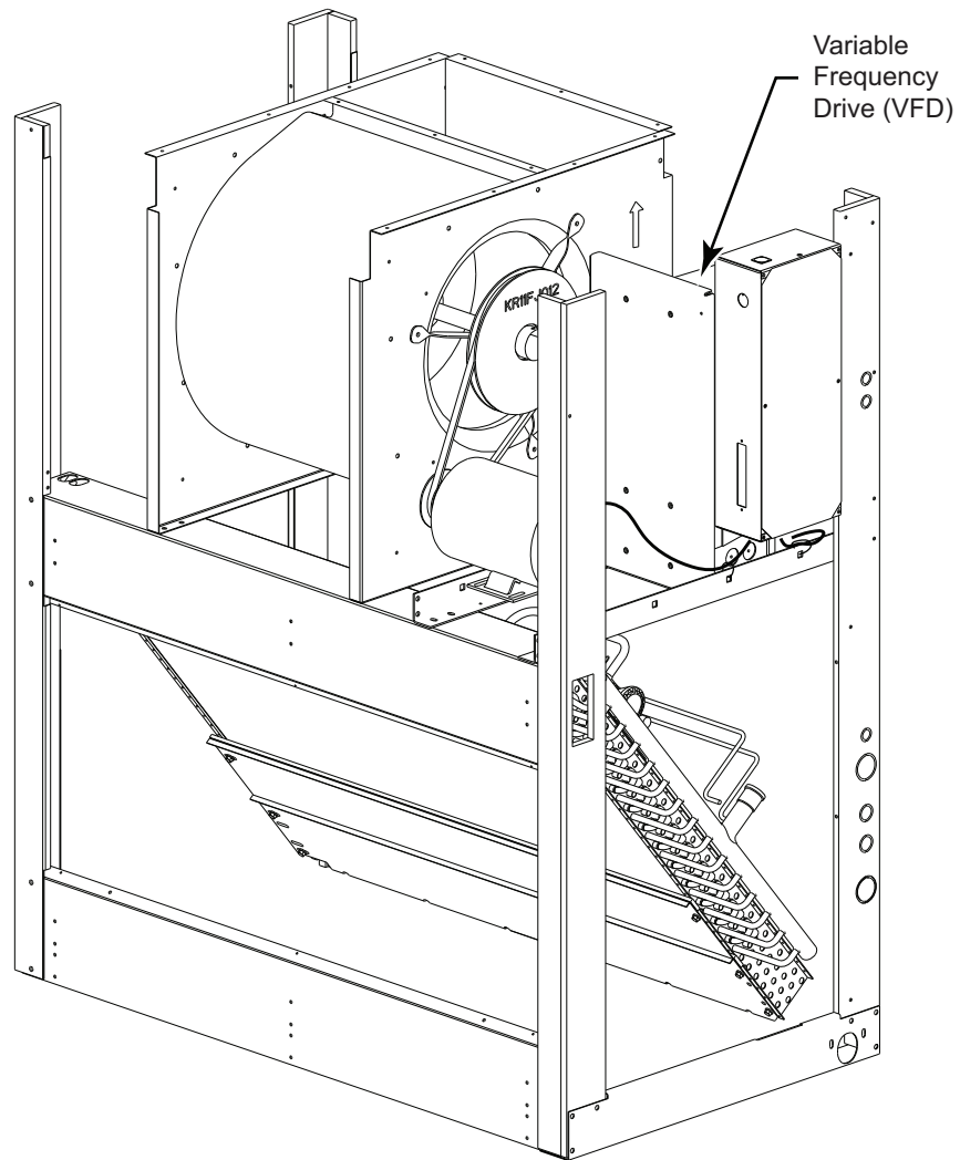
Fig. 21 — ACH550/580 VFD Location for the following units: 40RUA/RUQ 07-12, 40RUS 08-12 (575V only)
