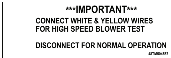
Fig. 24 — High Speed Test Label
