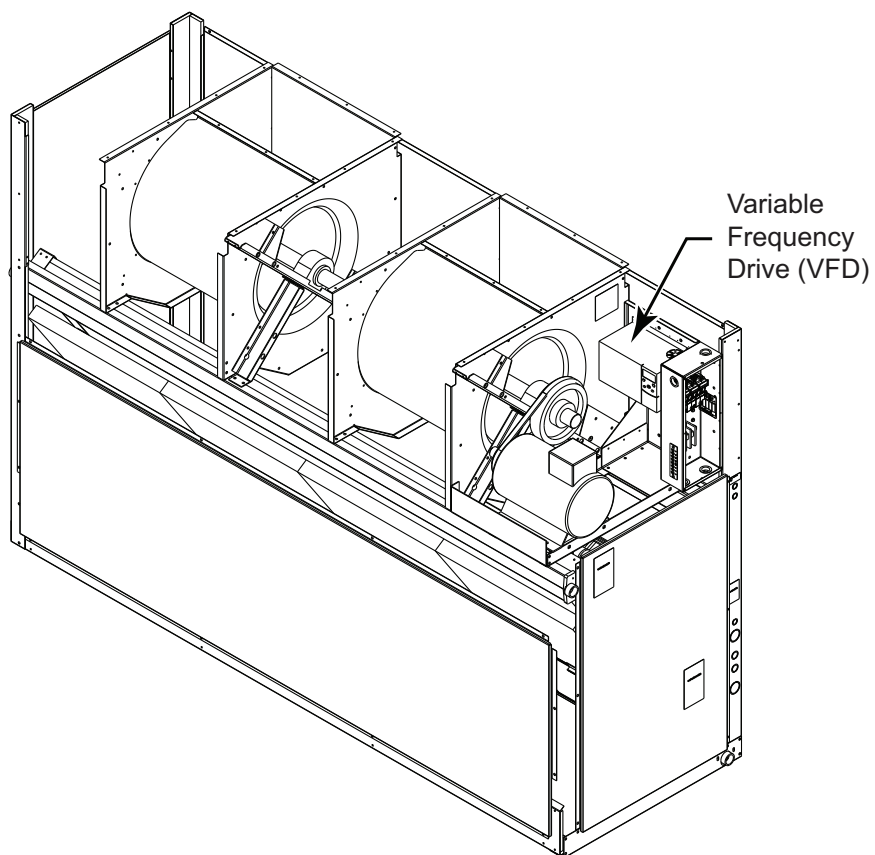
Fig. 20 — ACS320 VFD Location for the following units: 40RUA/RUS 28-30 (208/230V and 460V only)
