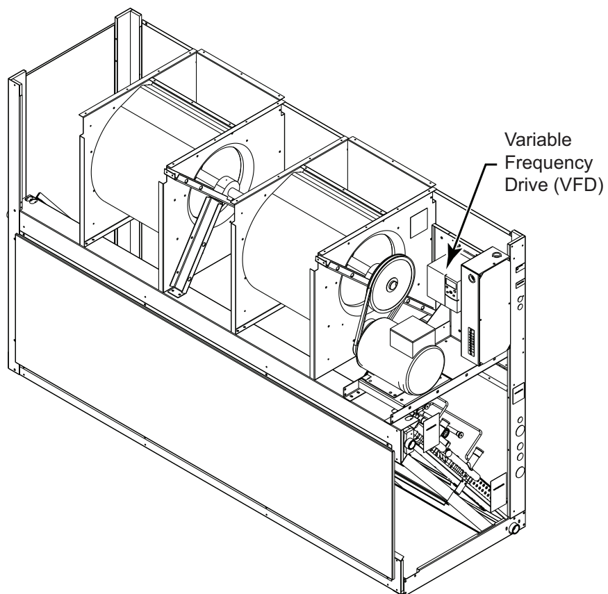
Fig. 19 — ACS320 VFD Location for the following units: 40RUA/RUS 14-25, 40RUQ 16-25 (208/230V and 460V only)
